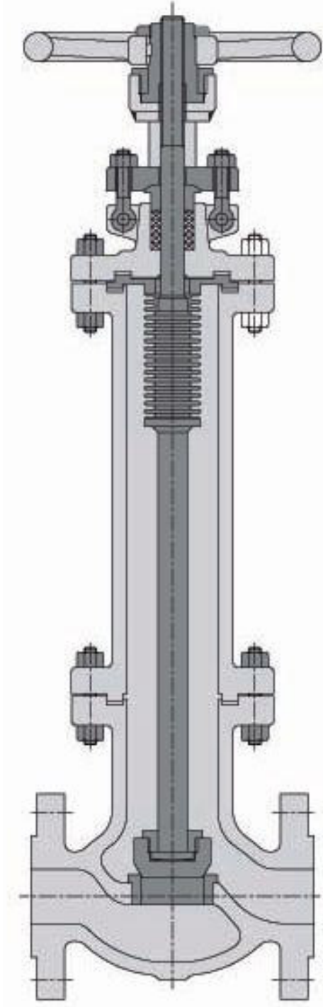
BELLOW SEAL "CRYOGENIC VALVE"
