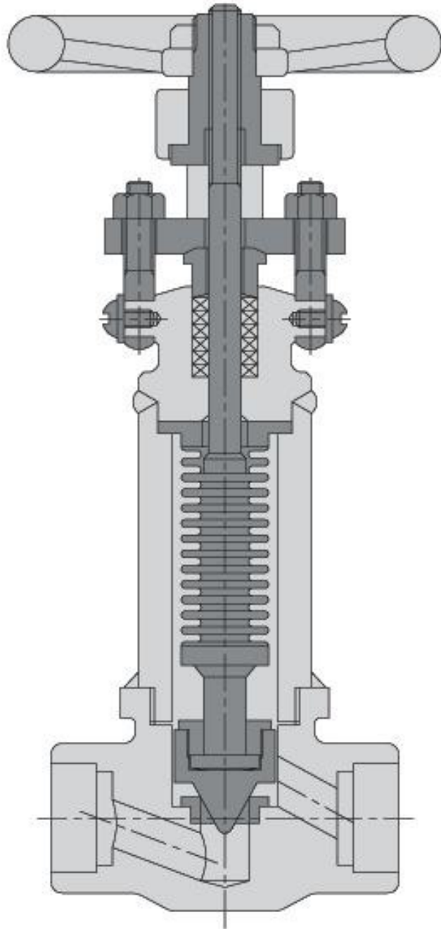
BELLOW SEAL "NEEDLE VALVE"
