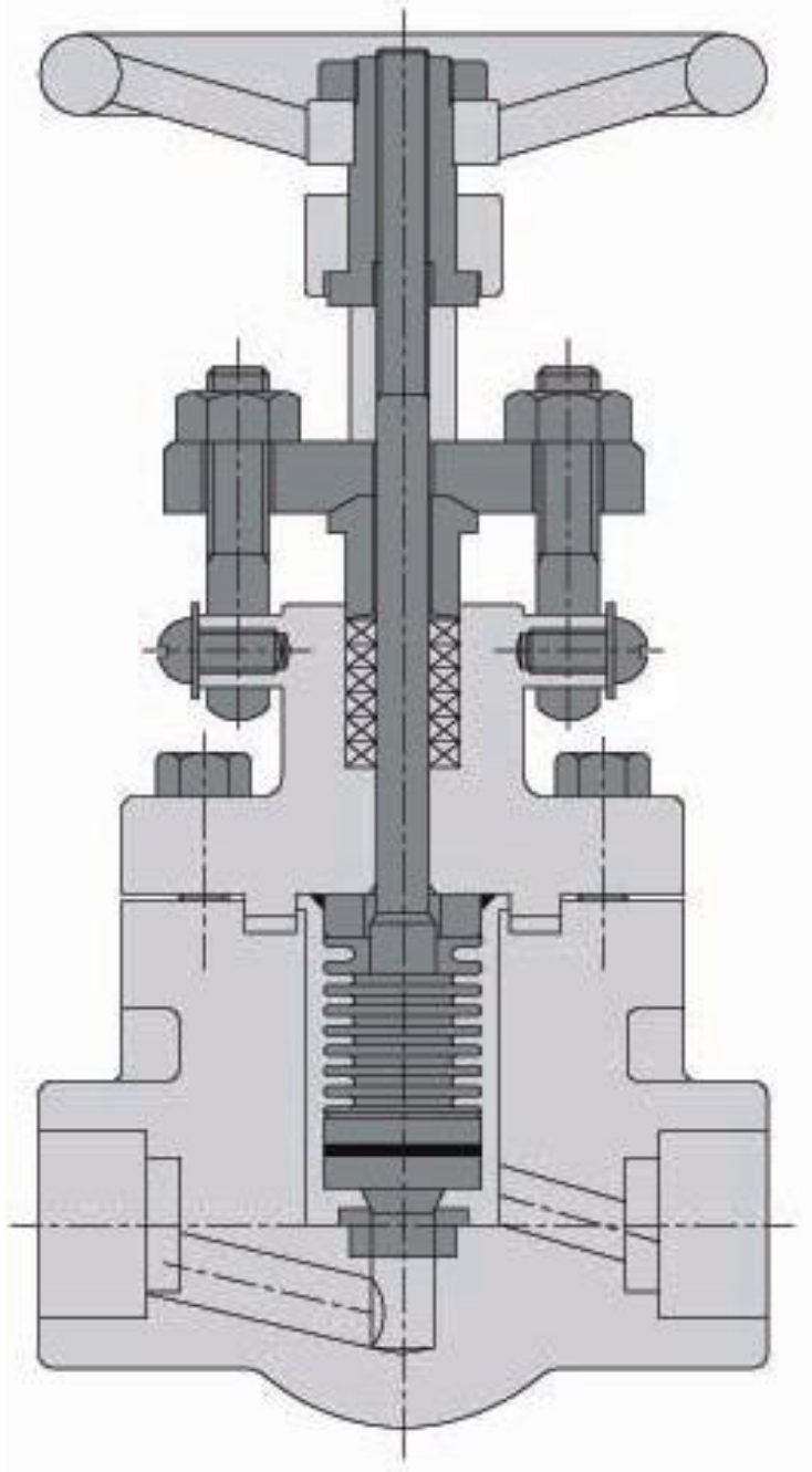
BELLOW SEAL "COMPACT DESIGN VALVE"
